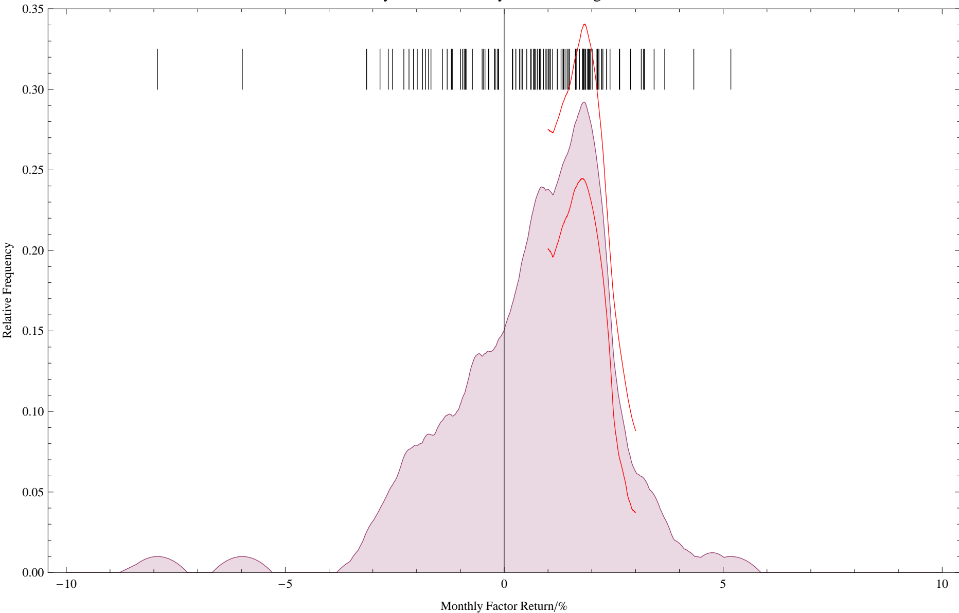
Kernel Density Estimates for Dynamic Trading Risk Factor Data
